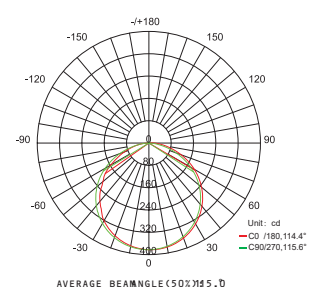
Photometric Diagram
